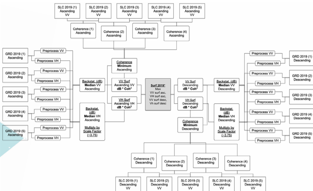
Flow chart for processing Sentinel-1 involving several images and processing methods.
